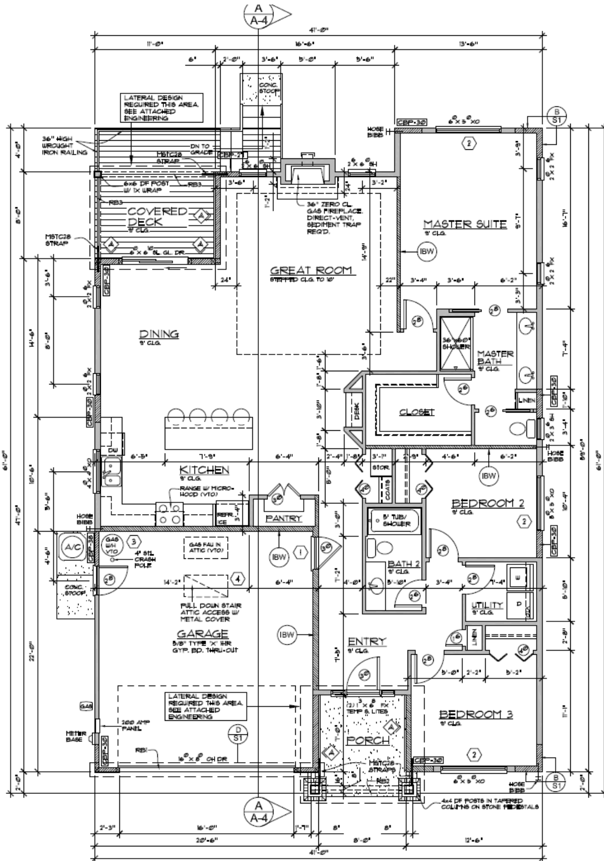
FLOOR PLAN 1/4" = 1'-0"
